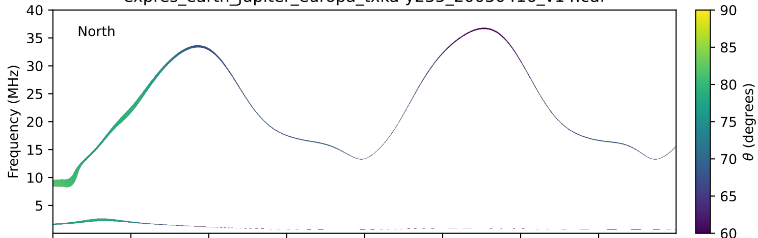
expres_earth_jupiter_europa_txka-y235_20030416_v14.cdf
