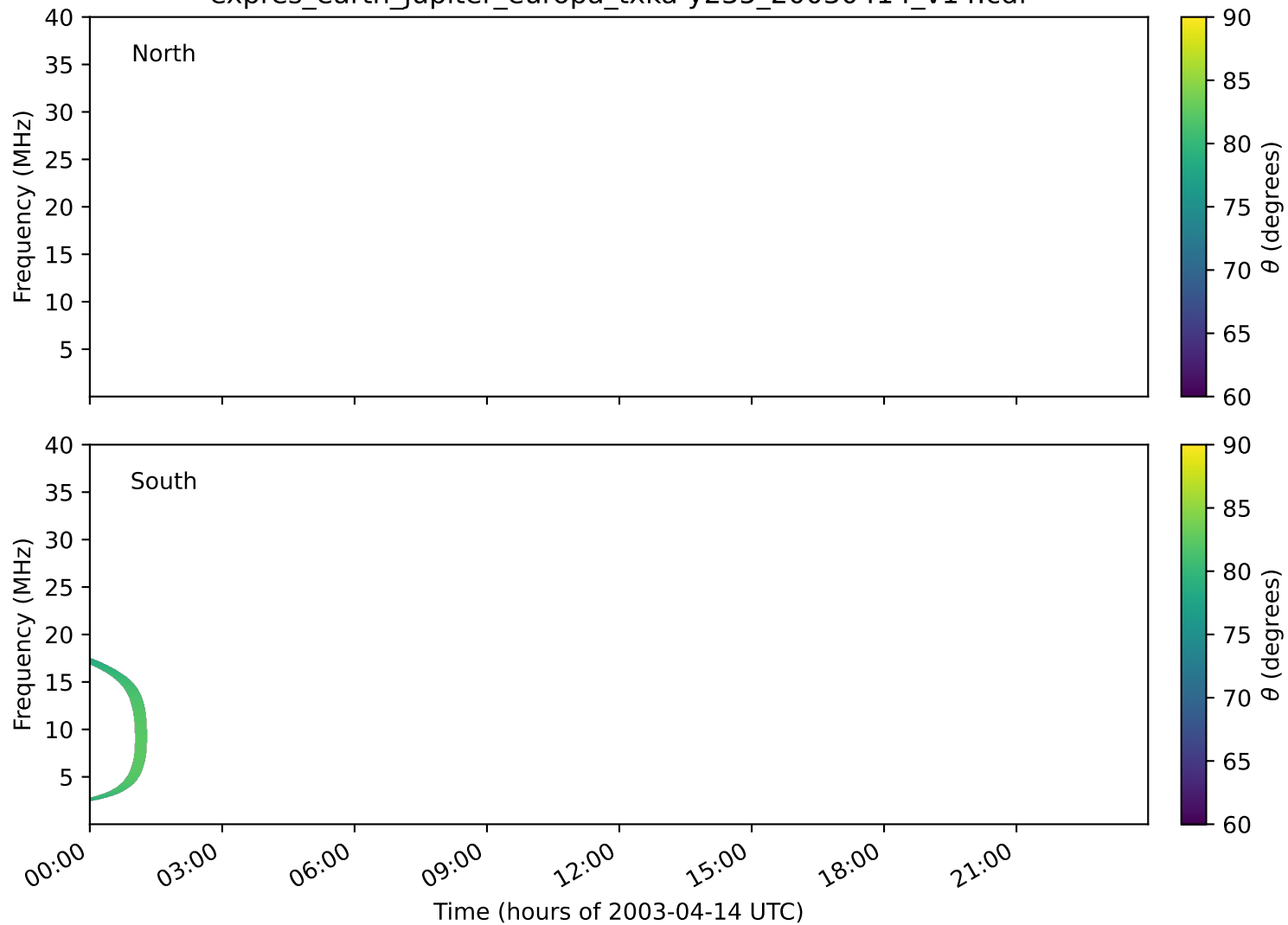
expres_earth_jupiter_europa_txka-y235_20030414_v14.cdf
