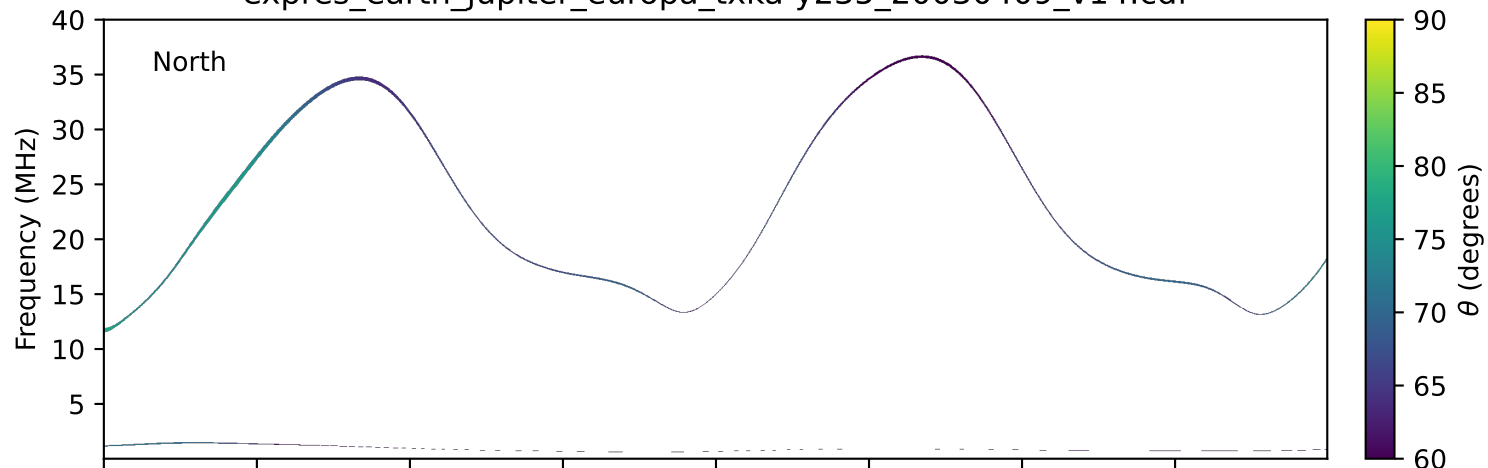
expres_earth_jupiter_europa_txka-y235_20030409_v14.cdf
