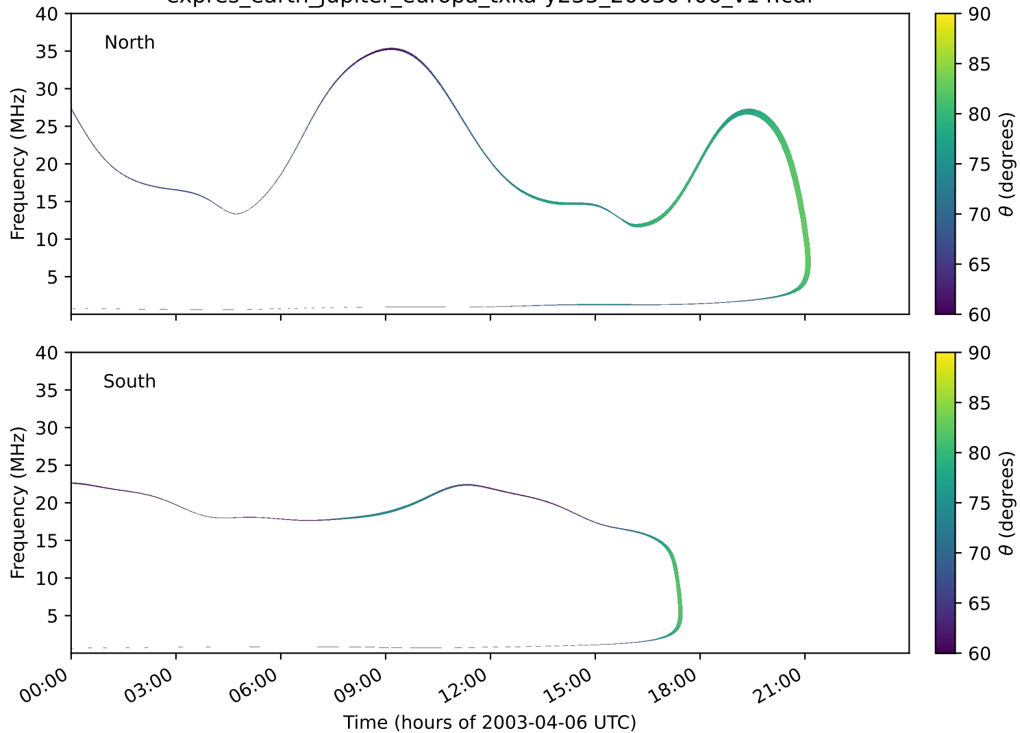
expres_earth_jupiter_europa_txka-y235_20030406_v14.cdf
