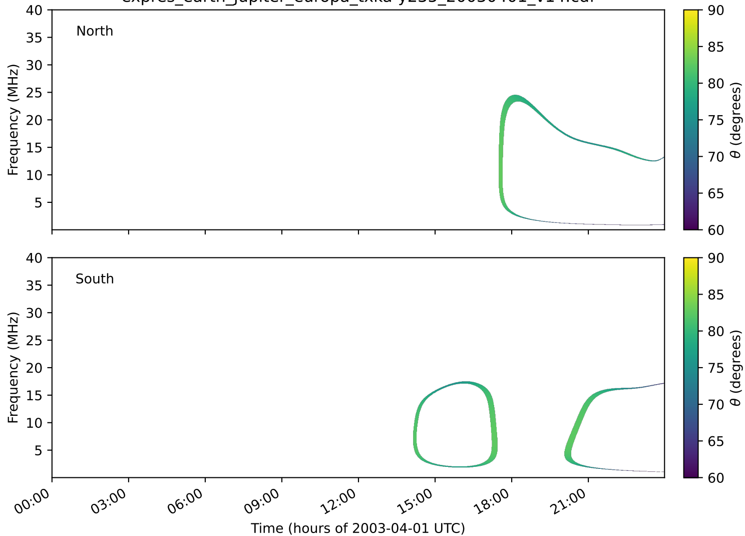
expres_earth_jupiter_europa_txka-y235_20030401_v14.cdf
