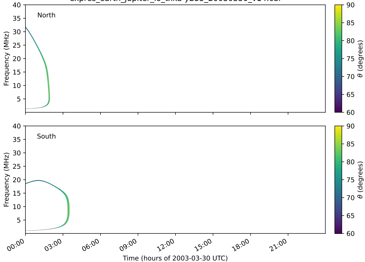
expres_earth_jupiter_io_txka-y235_20030330_v14.cdf
