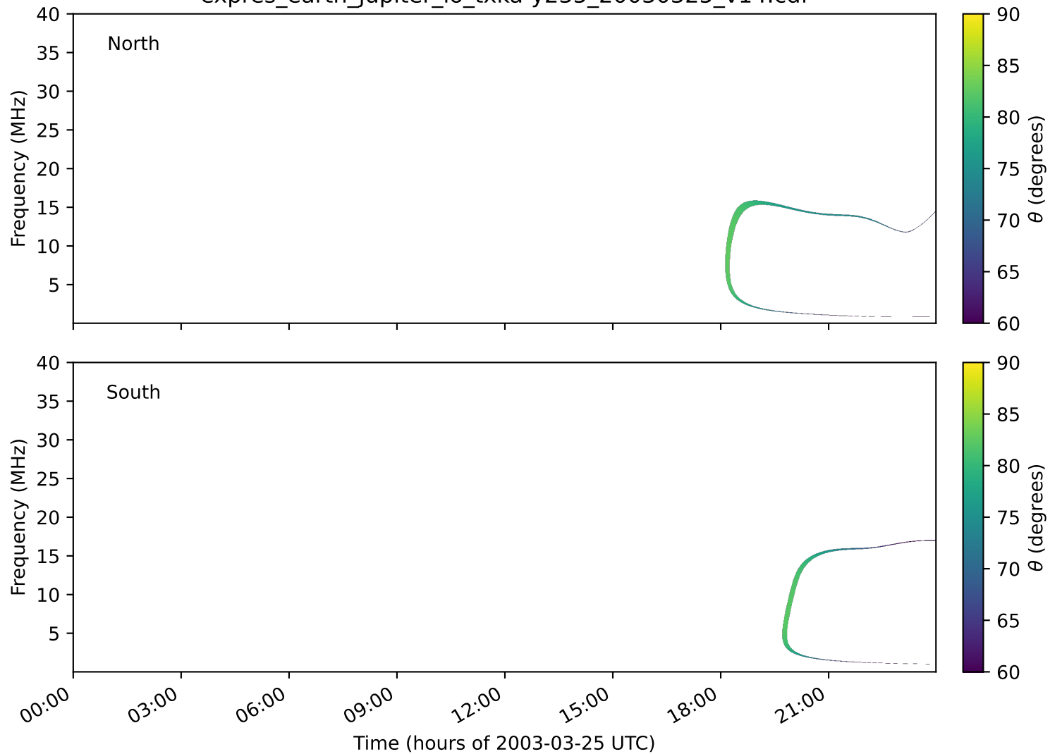
expres_earth_jupiter_io_txka-y235_20030325_v14.cdf
