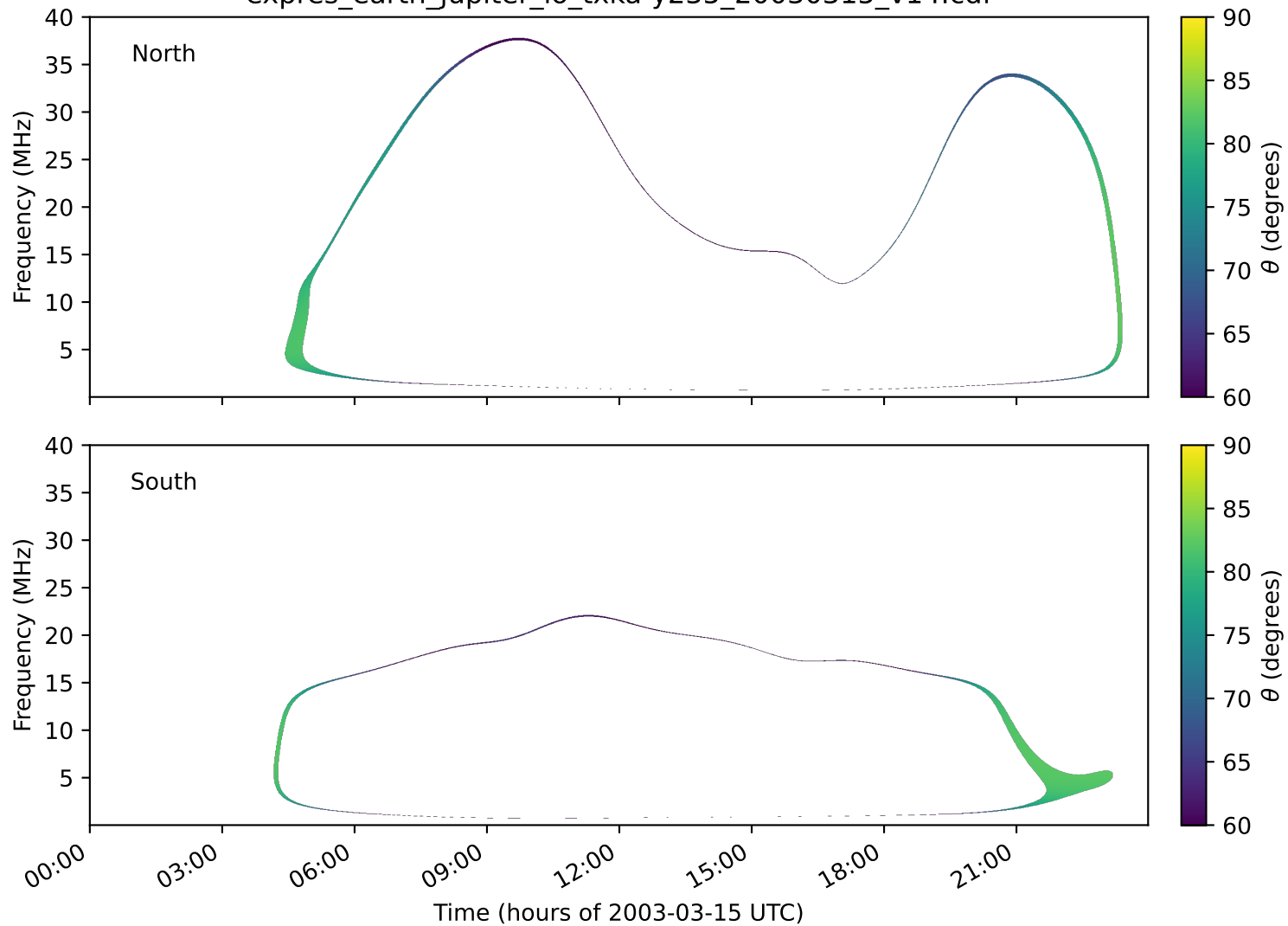
expres_earth_jupiter_io_txka-y235_20030315_v14.cdf
