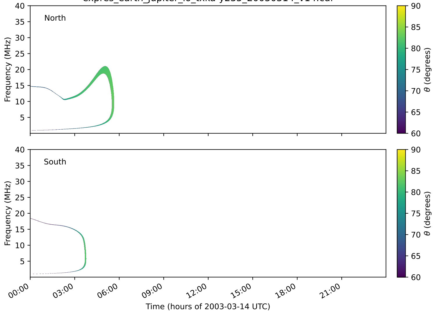
expres_earth_jupiter_io_txka-y235_20030314_v14.cdf
