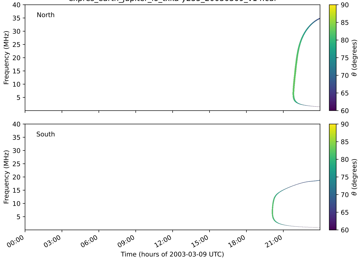
expres_earth_jupiter_io_txka-y235_20030309_v14.cdf
