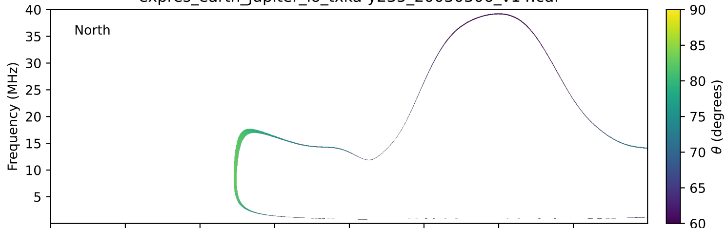
expres_earth_jupiter_io_txka-y235_20030306_v14.cdf
