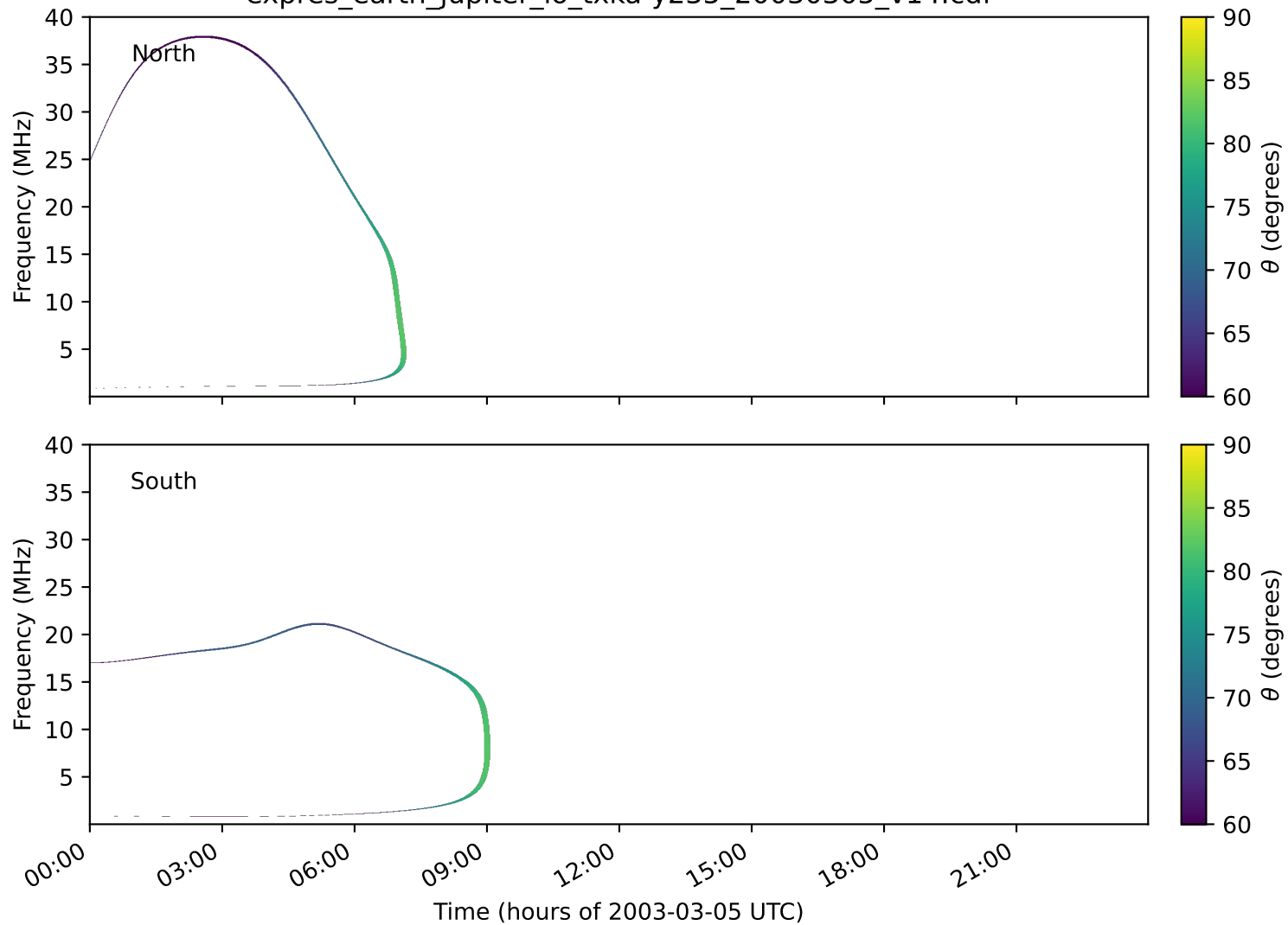
expres_earth_jupiter_io_txka-y235_20030305_v14.cdf
