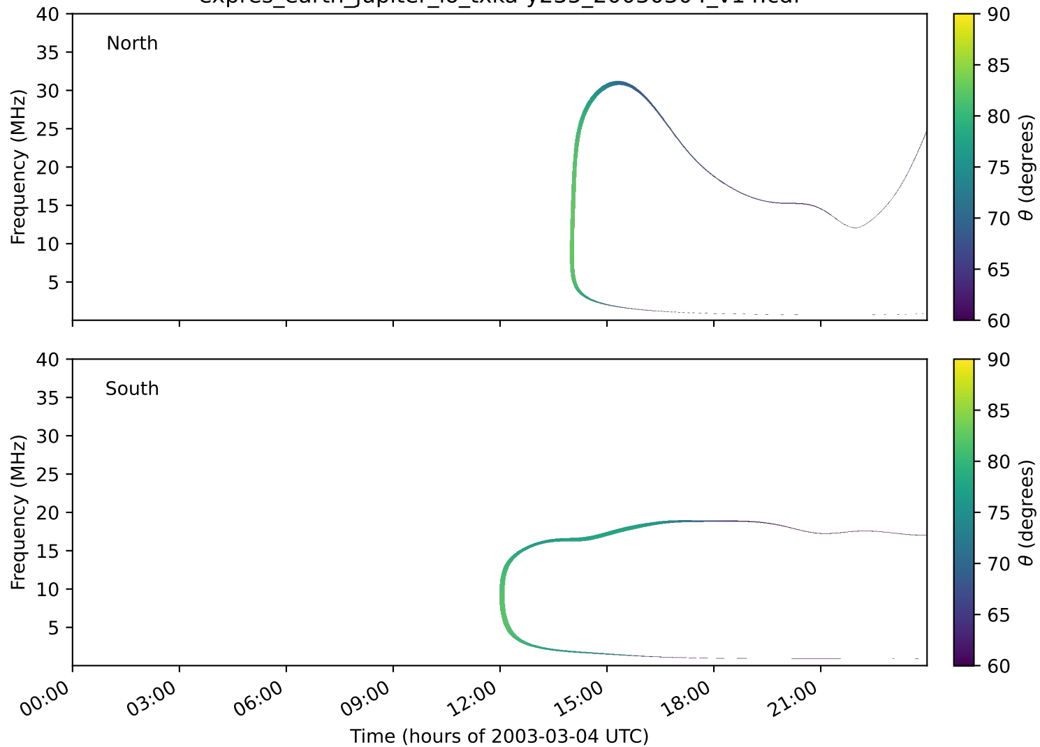
expres_earth_jupiter_io_txka-y235_20030304_v14.cdf
