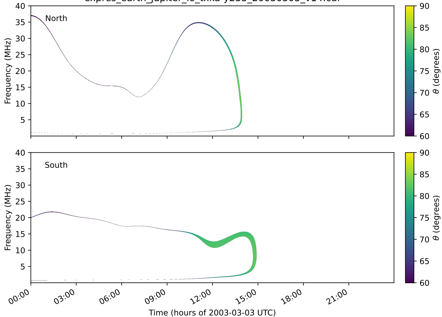
expres_earth_jupiter_io_txka-y235_20030303_v14.cdf
