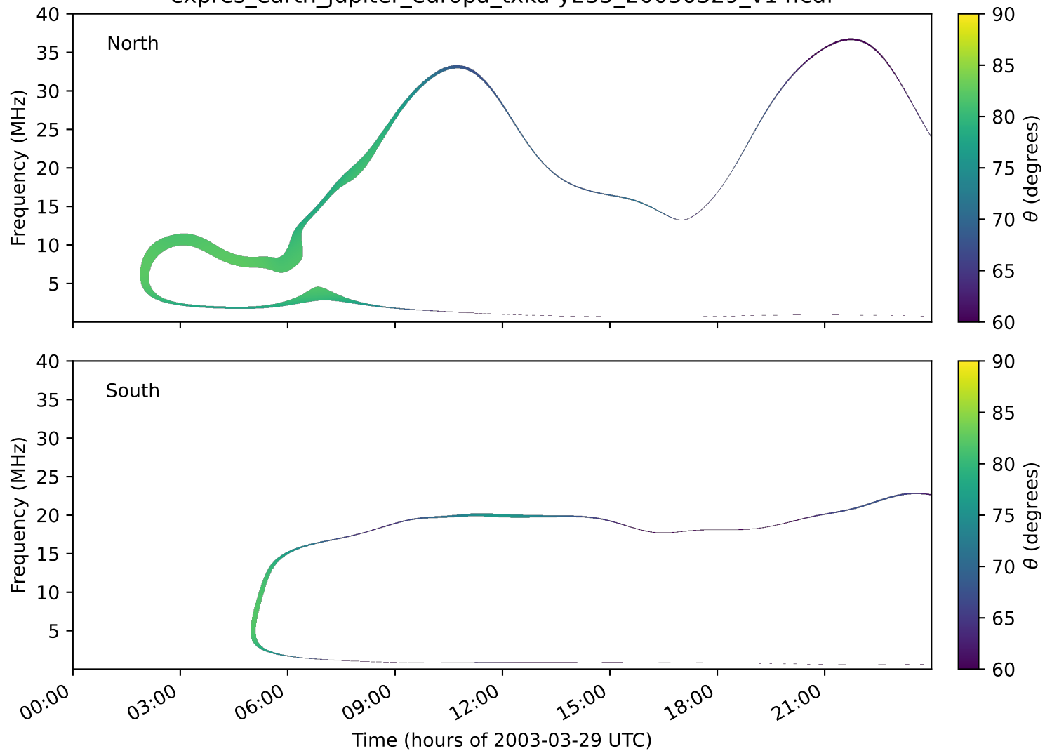
expres_earth_jupiter_europa_txka-y235_20030329_v14.cdf
