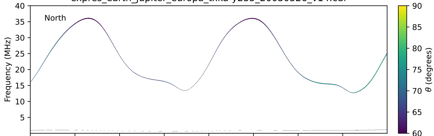
expres_earth_jupiter_europa_txka-y235_20030326_v14.cdf
