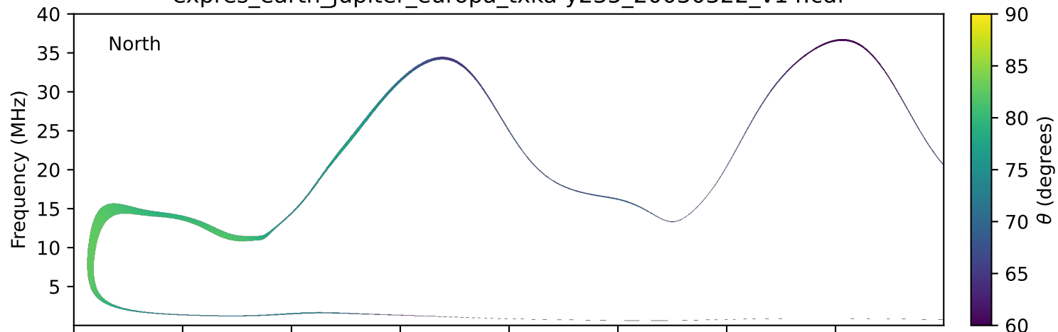
expres_earth_jupiter_europa_txka-y235_20030322_v14.cdf
