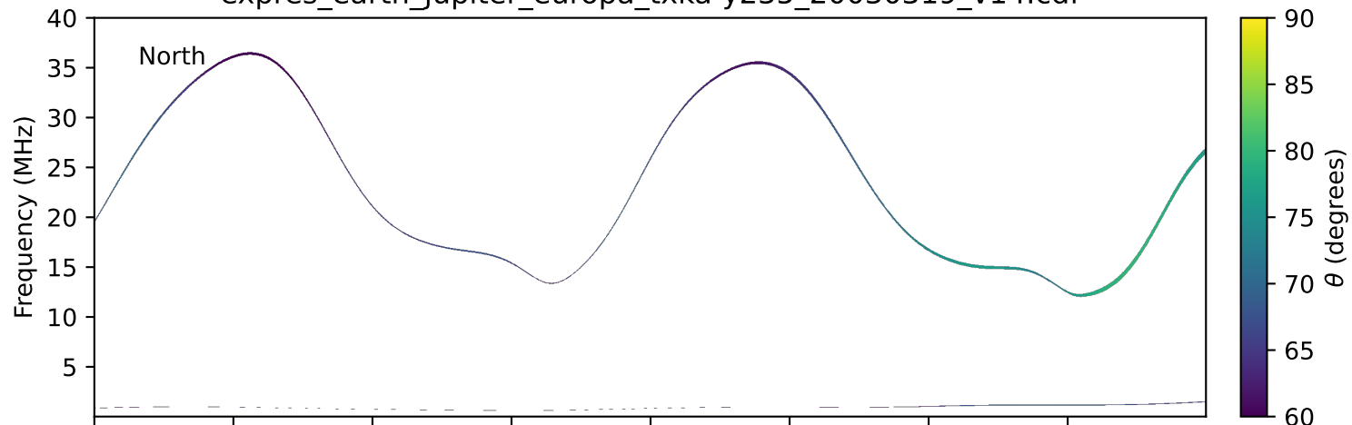
expres_earth_jupiter_europa_txka-y235_20030319_v14.cdf
