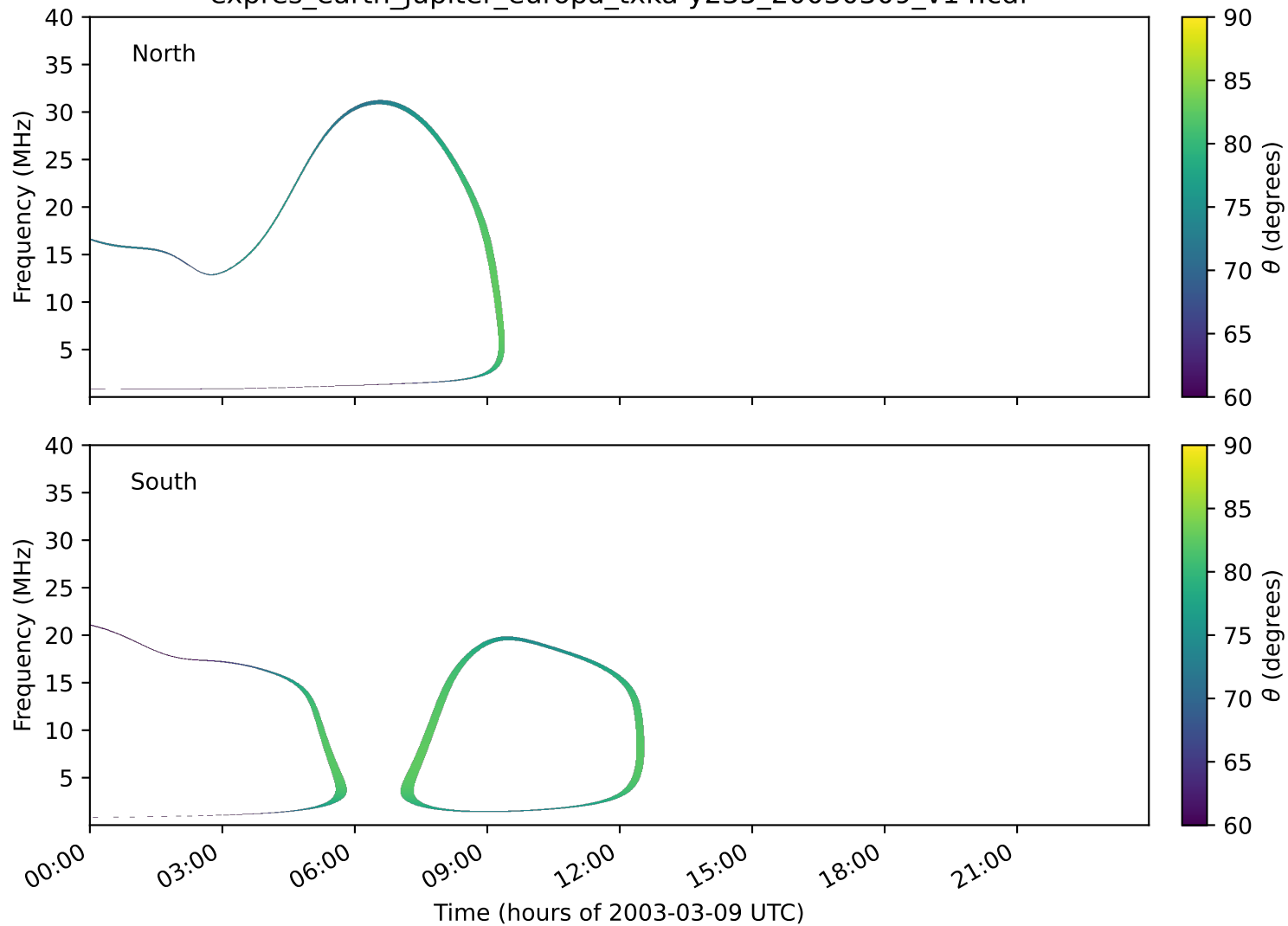
expres_earth_jupiter_europa_txka-y235_20030309_v14.cdf
