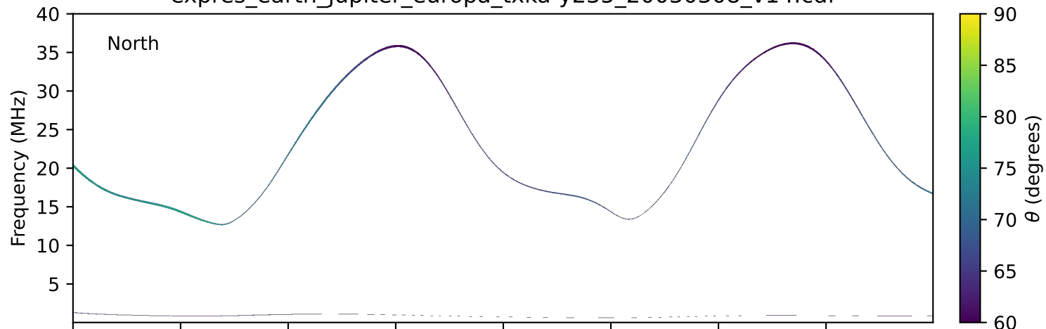
expres_earth_jupiter_europa_txka-y235_20030308_v14.cdf
