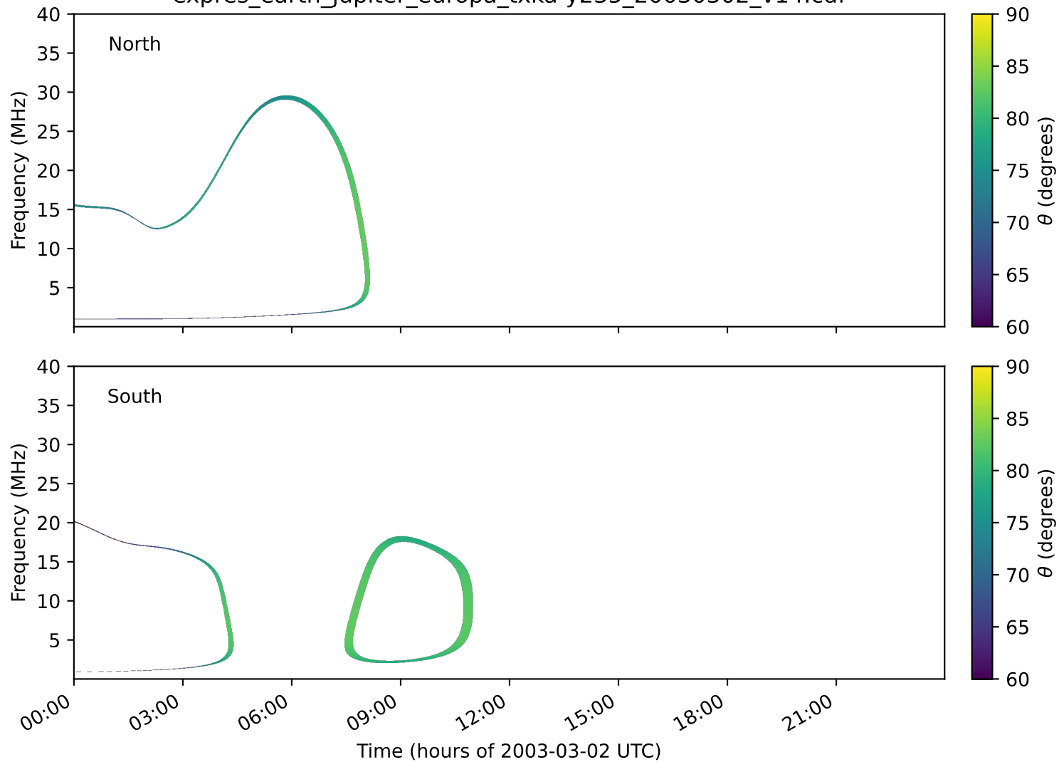
expres_earth_jupiter_europa_txka-y235_20030302_v14.cdf
