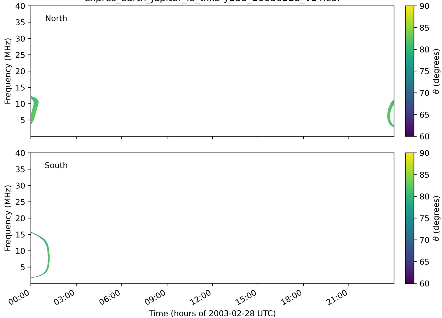
expres_earth_jupiter_io_txka-y235_20030228_v14.cdf
