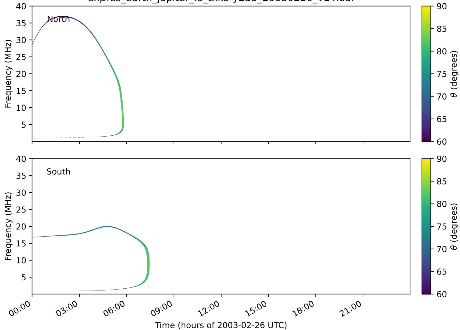
expres_earth_jupiter_io_txka-y235_20030226_v14.cdf
