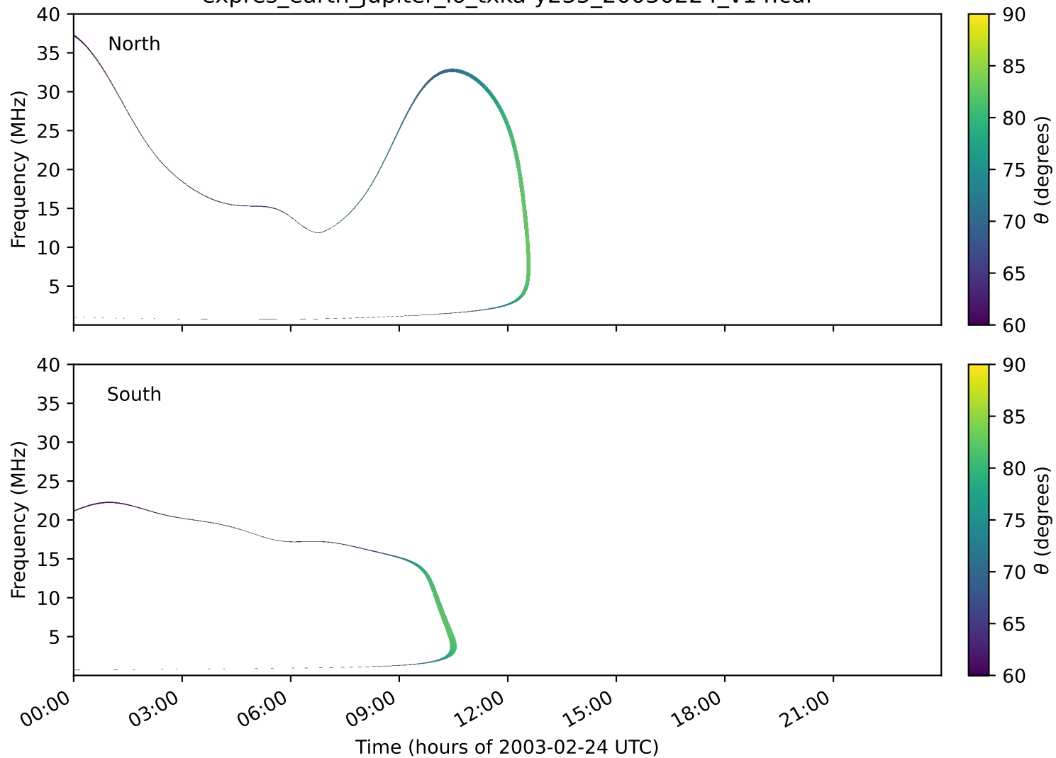
expres_earth_jupiter_io_txka-y235_20030224_v14.cdf
