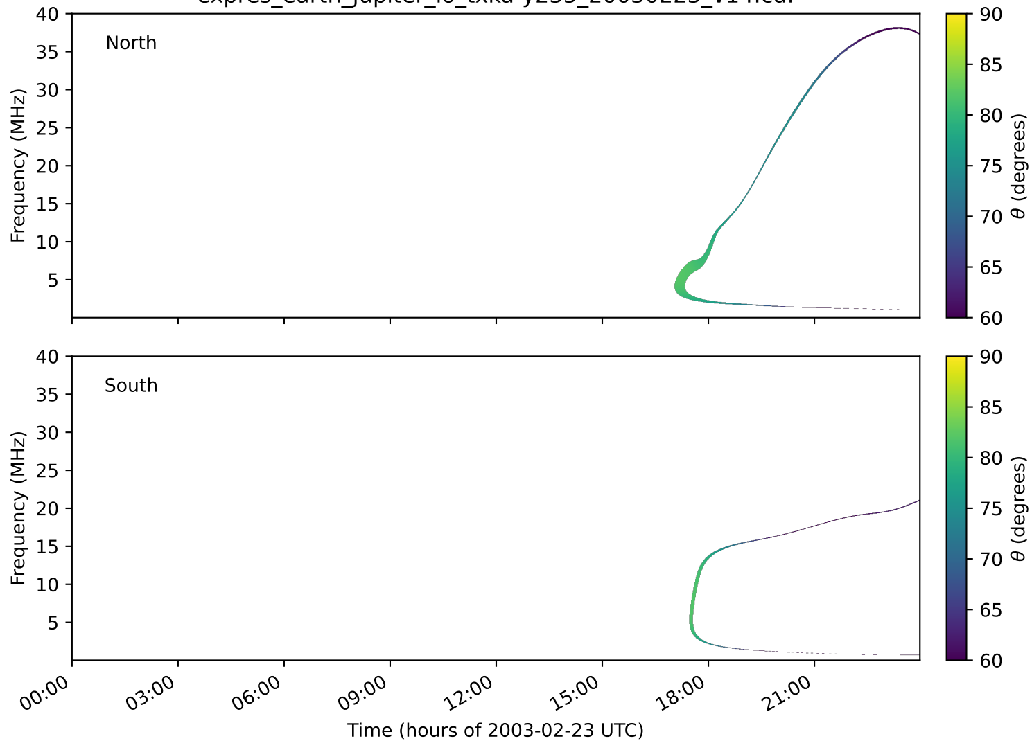
expres_earth_jupiter_io_txka-y235_20030223_v14.cdf
