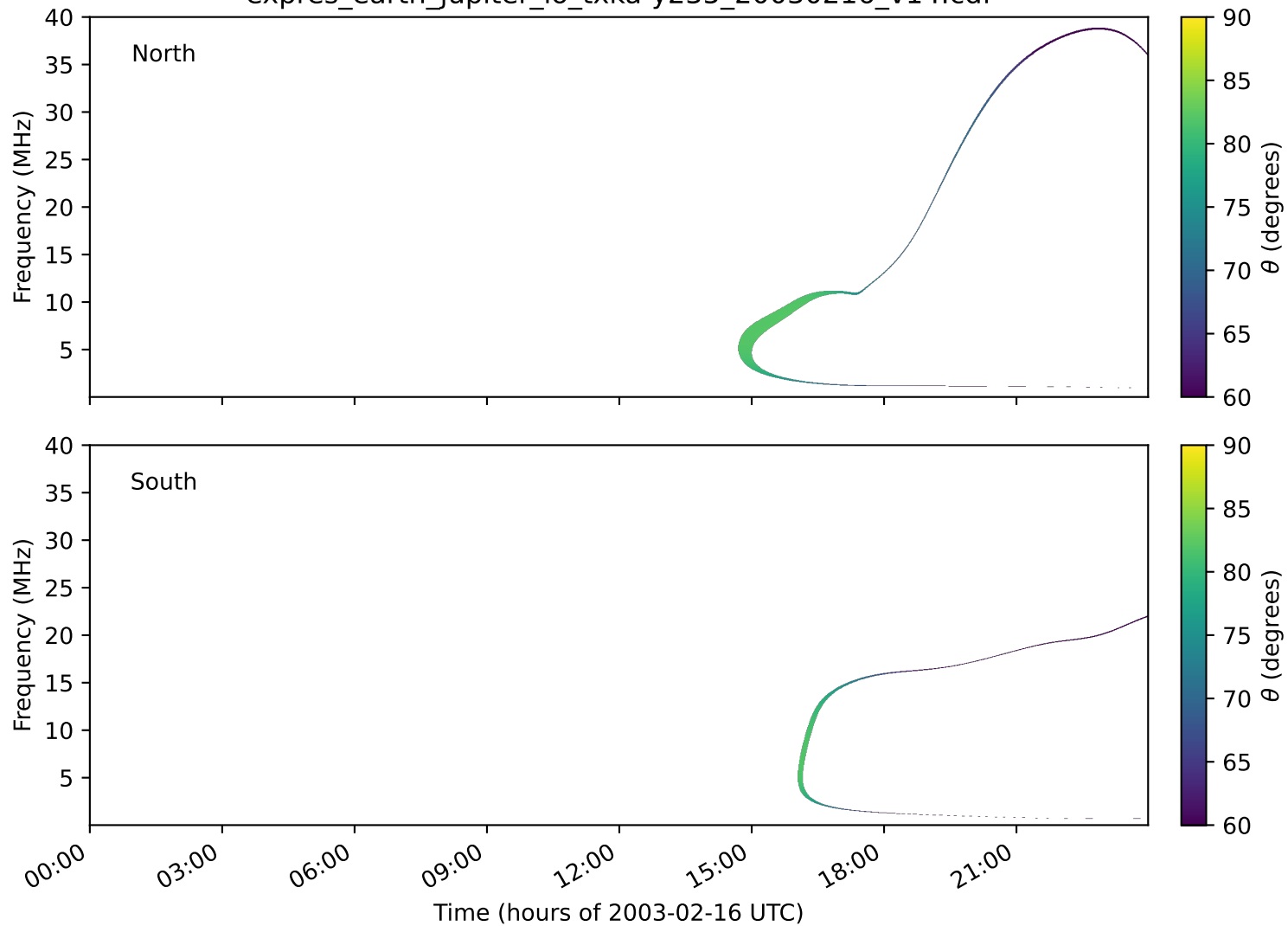
expres_earth_jupiter_io_txka-y235_20030216_v14.cdf
