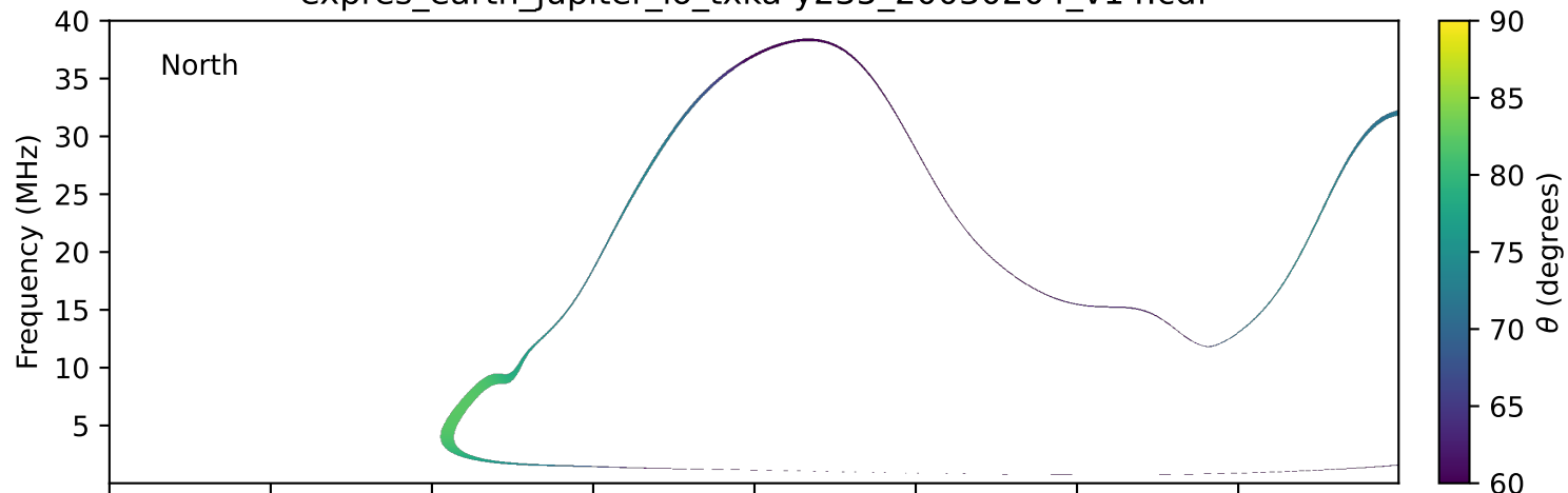
expres_earth_jupiter_io_txka-y235_20030204_v14.cdf
