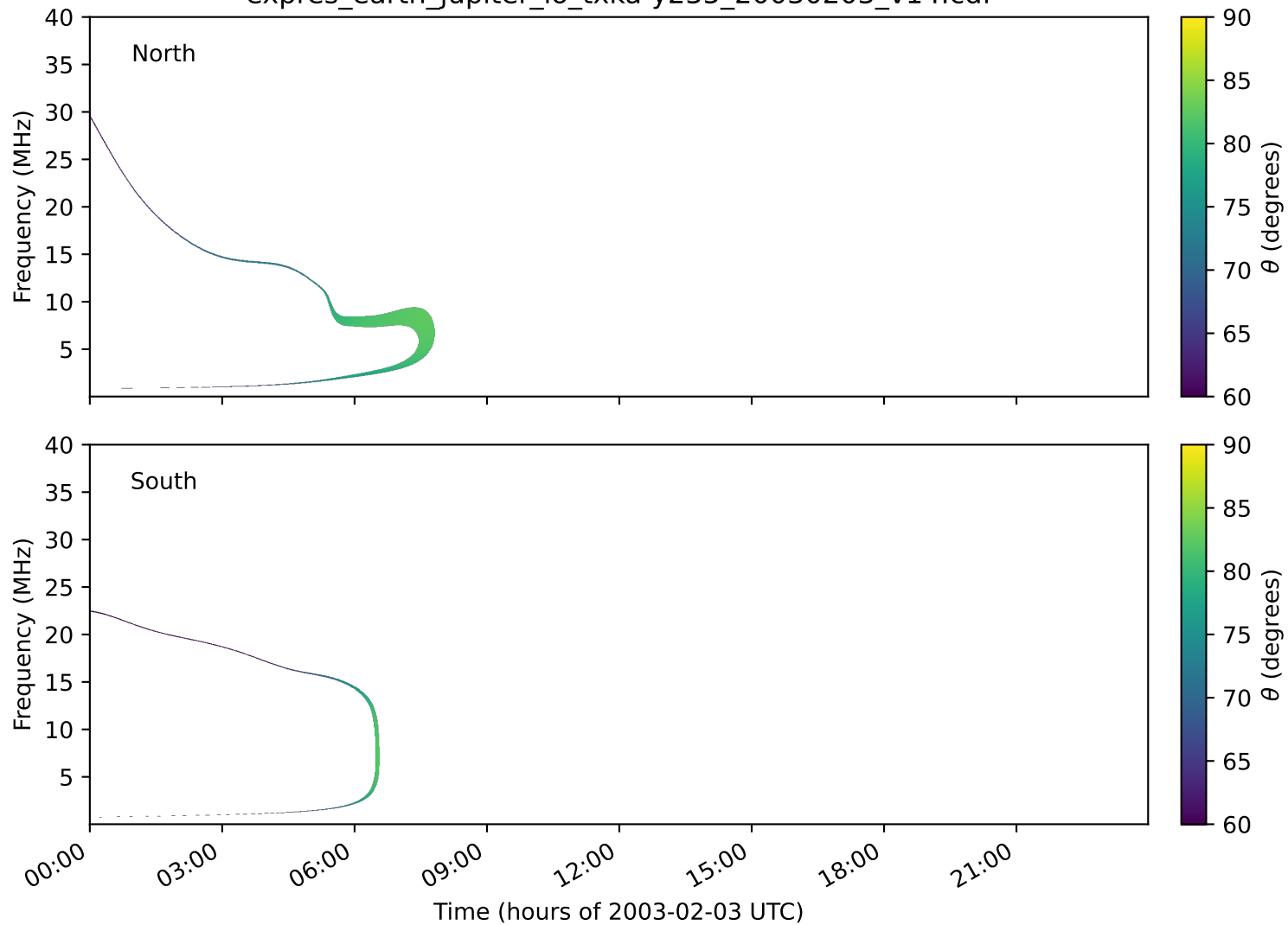
expres_earth_jupiter_io_txka-y235_20030203_v14.cdf
