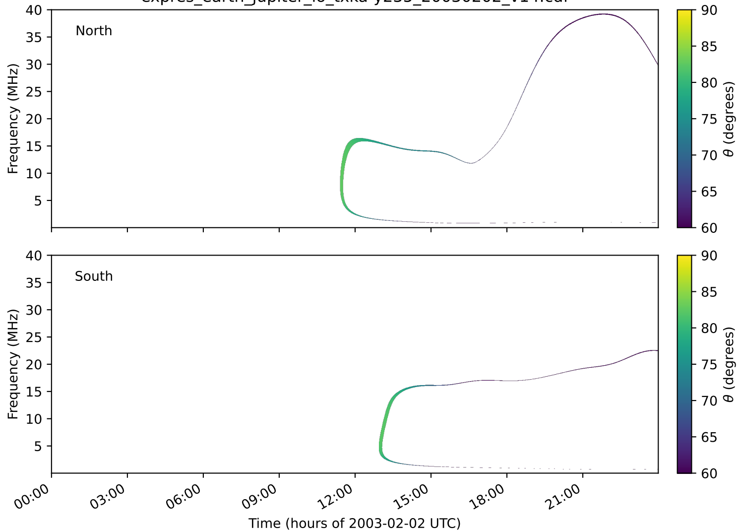
expres_earth_jupiter_io_txka-y235_20030202_v14.cdf
