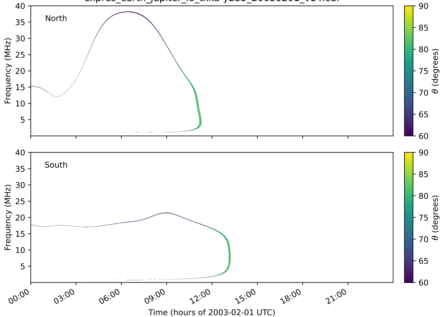
expres_earth_jupiter_io_txka-y235_20030201_v14.cdf
