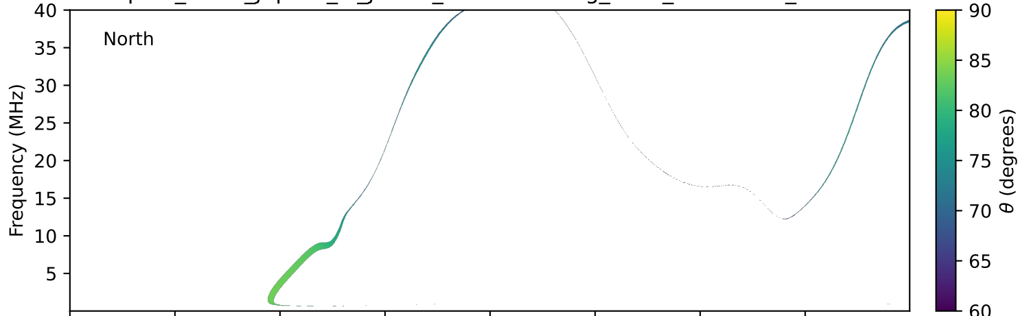
expres_earth_jupiter_io_jrm33_lossc-wid1deg_3kev_20030204_v11.cdf
