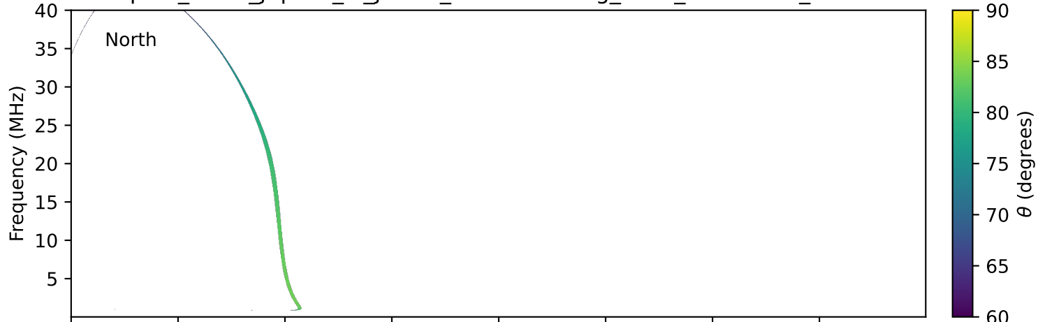
expres_earth_jupiter_io_jrm09_lossc-wid1deg_3kev_20030226_v11.cdf
