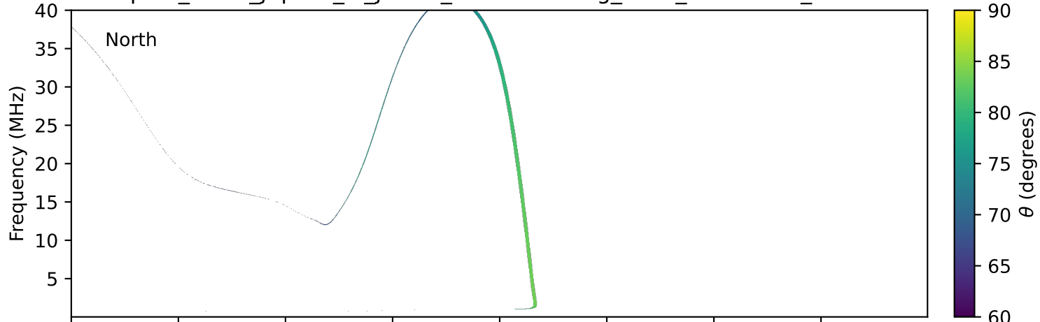
expres_earth_jupiter_io_jrm09_lossc-wid1deg_3kev_20030224_v11.cdf
