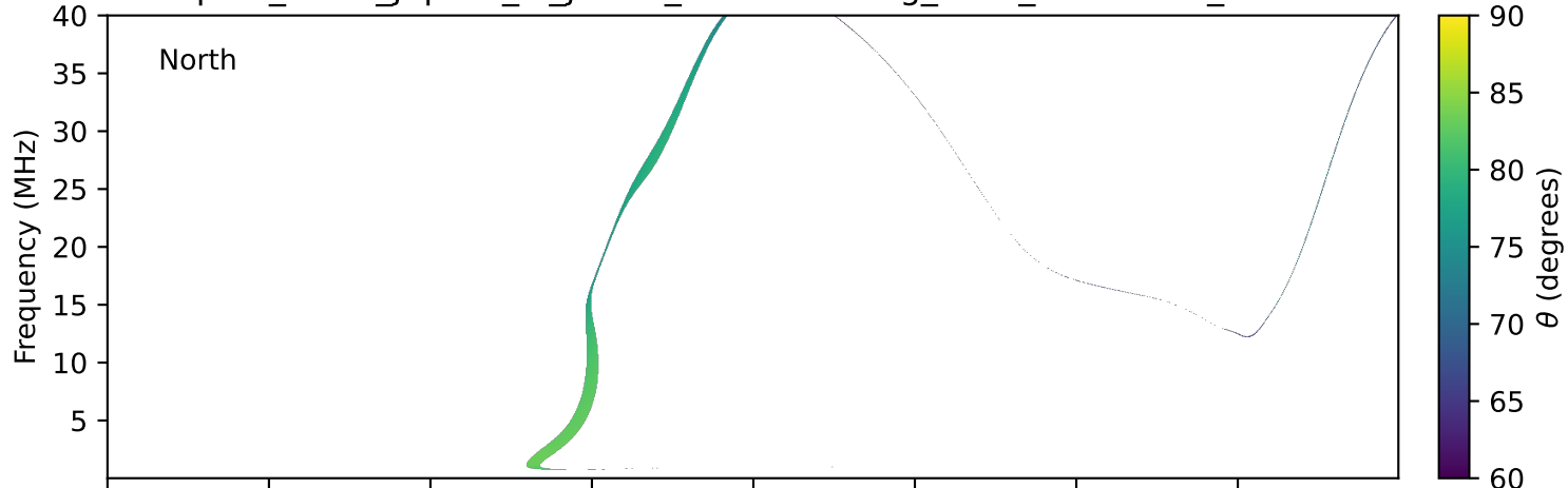
expres_earth_jupiter_io_jrm09_lossc-wid1deg_3kev_20030211_v11.cdf
