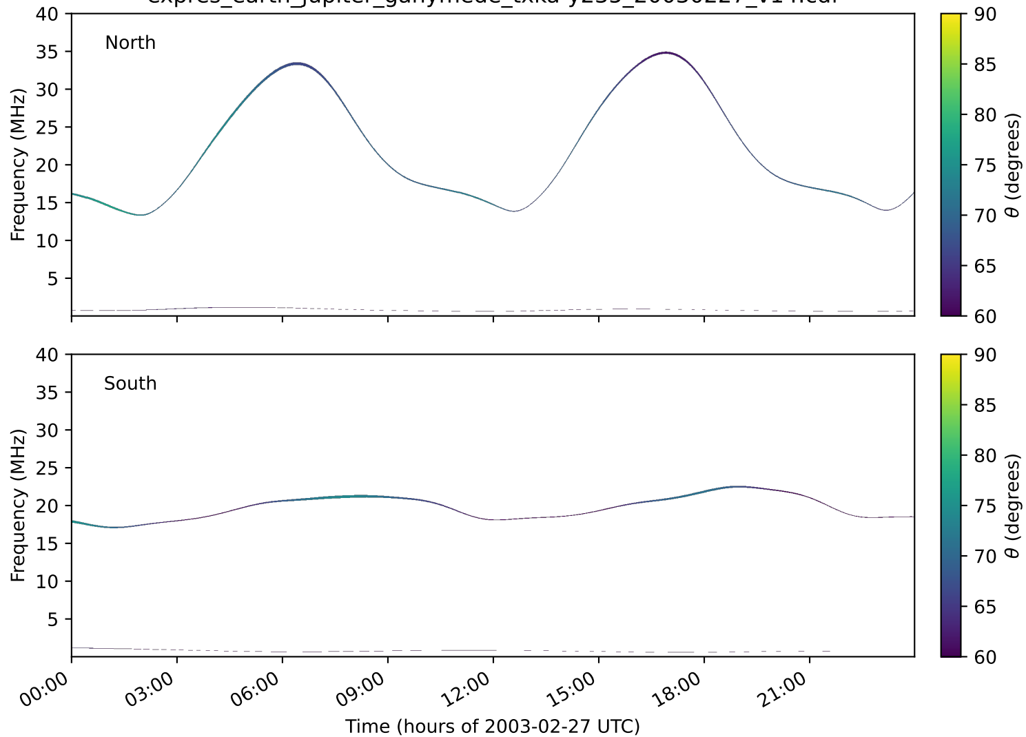
expres_earth_jupiter_ganymede_txka-y235_20030227_v14.cdf
