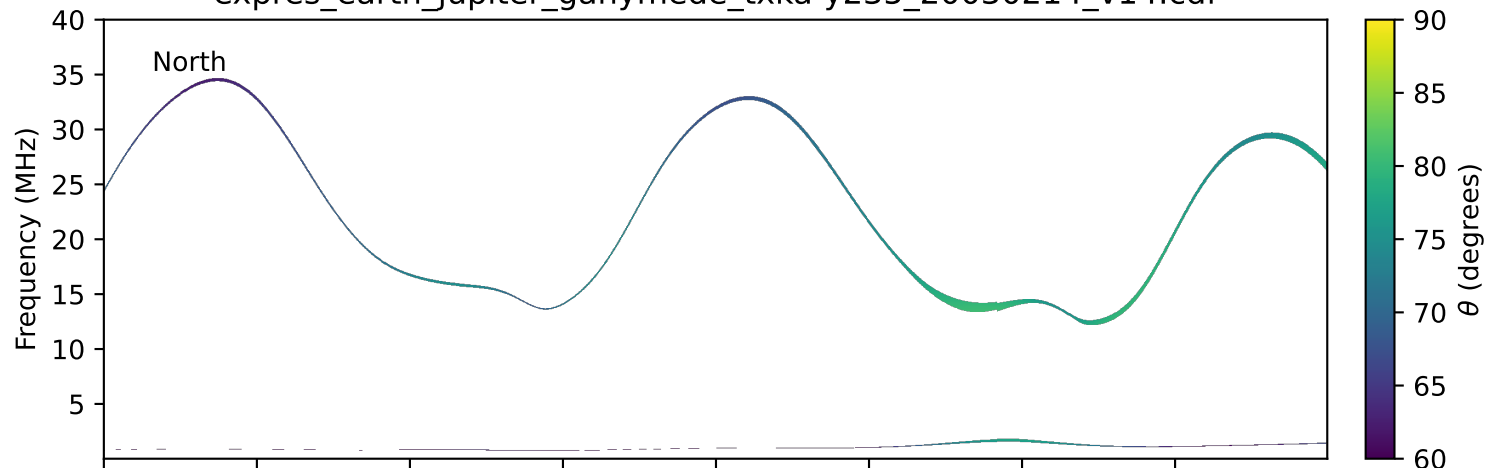
expres_earth_jupiter_ganymede_txka-y235_20030214_v14.cdf
