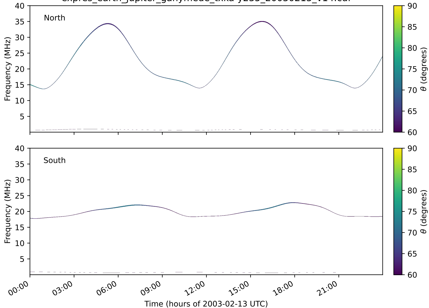
expres_earth_jupiter_ganymede_txka-y235_20030213_v14.cdf
