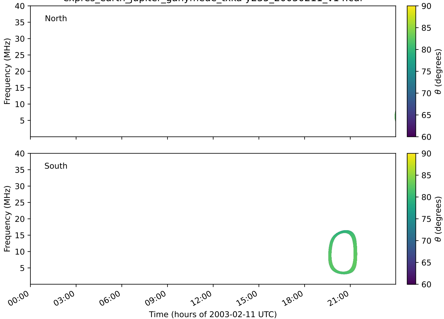
expres_earth_jupiter_ganymede_txka-y235_20030211_v14.cdf
