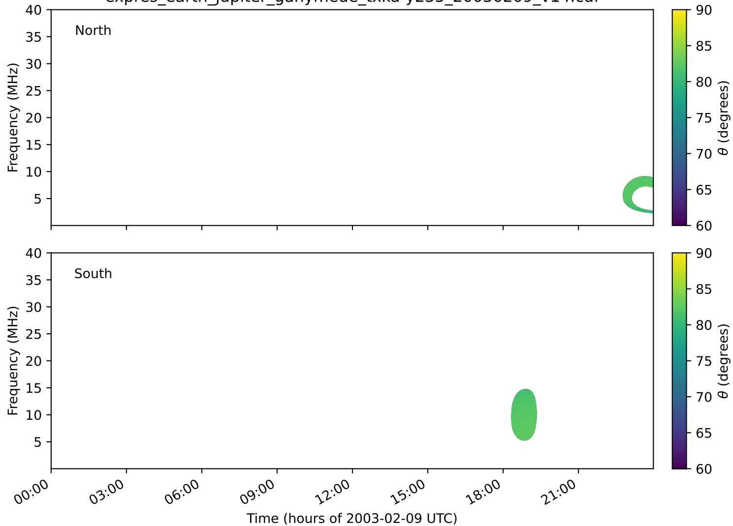
expres_earth_jupiter_ganymede_txka-y235_20030209_v14.cdf
