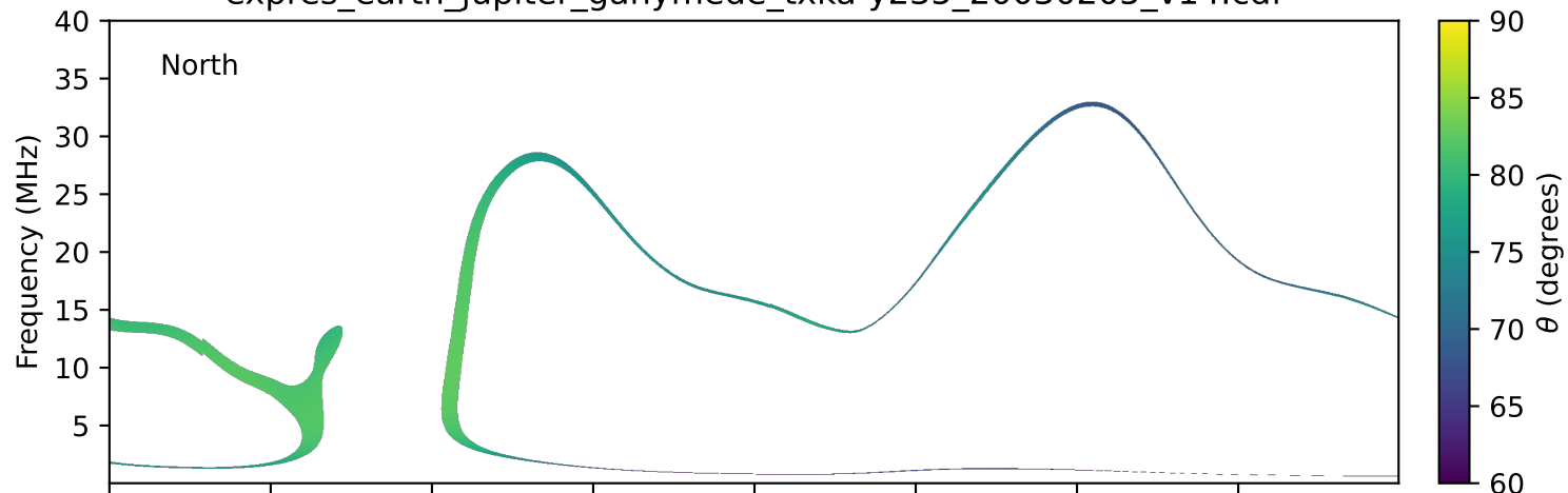
expres_earth_jupiter_ganymede_txka-y235_20030205_v14.cdf
