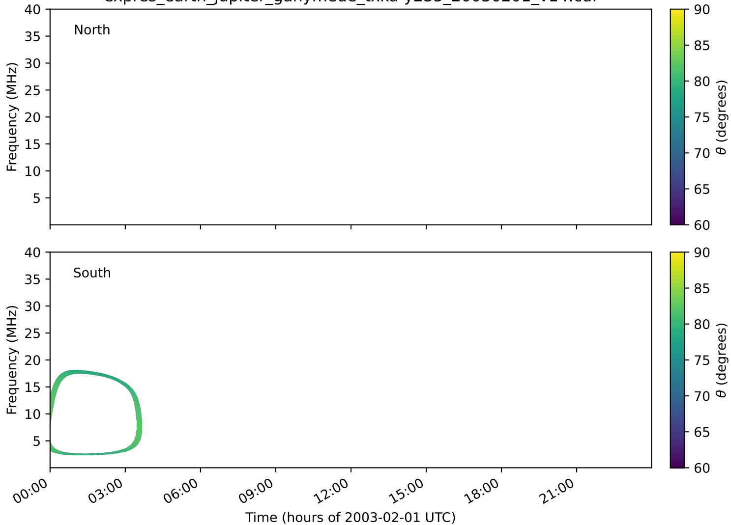
expres_earth_jupiter_ganymede_txka-y235_20030201_v14.cdf
