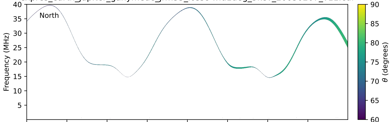
expres_earth_jupiter_ganymede_jrm33_lossc-wid1deg_3kev_20030207_v11.cdf
