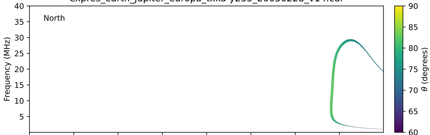
expres_earth_jupiter_europa_txka-y235_20030228_v14.cdf
