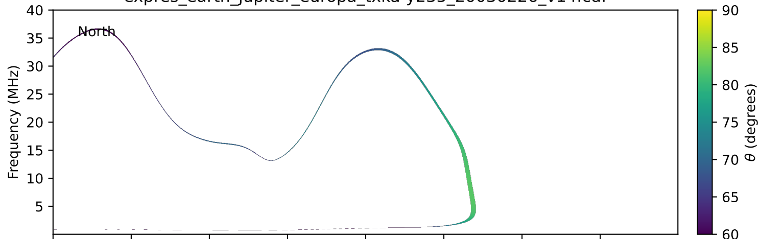
expres_earth_jupiter_europa_txka-y235_20030226_v14.cdf
