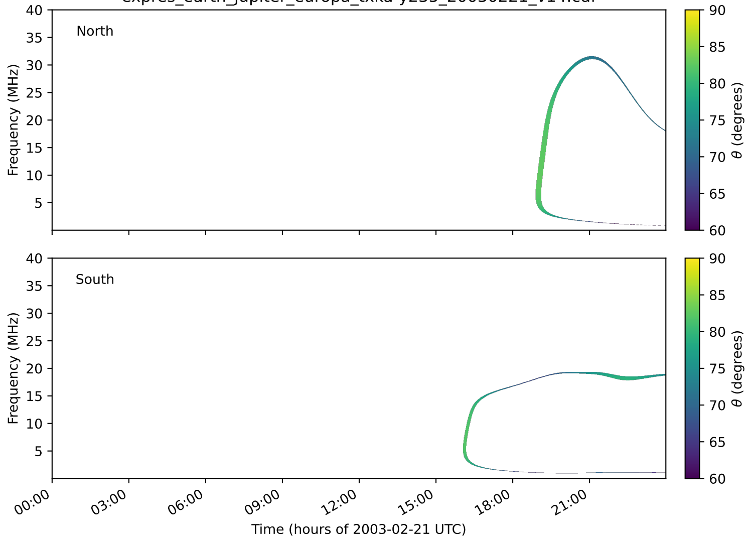
expres_earth_jupiter_europa_txka-y235_20030221_v14.cdf
