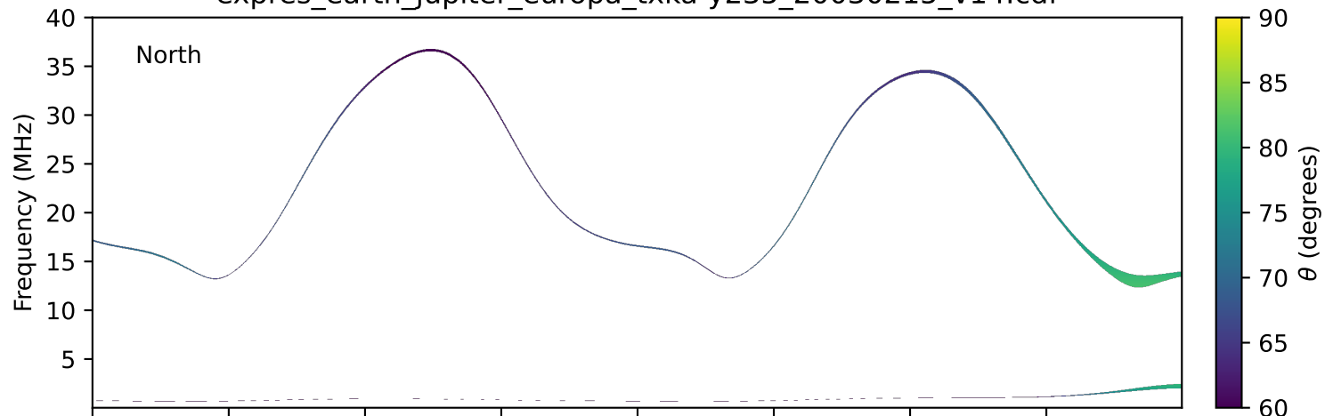
expres_earth_jupiter_europa_txka-y235_20030215_v14.cdf
