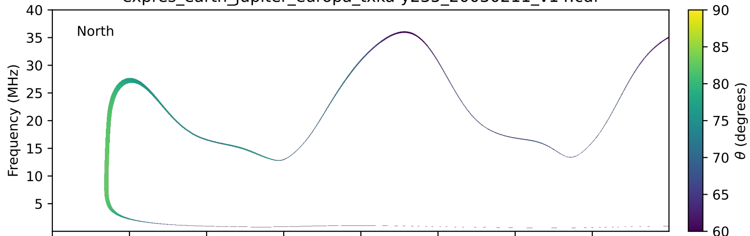
expres_earth_jupiter_europa_txka-y235_20030211_v14.cdf
