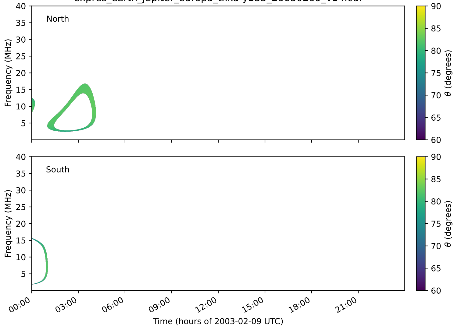
expres_earth_jupiter_europa_txka-y235_20030209_v14.cdf
