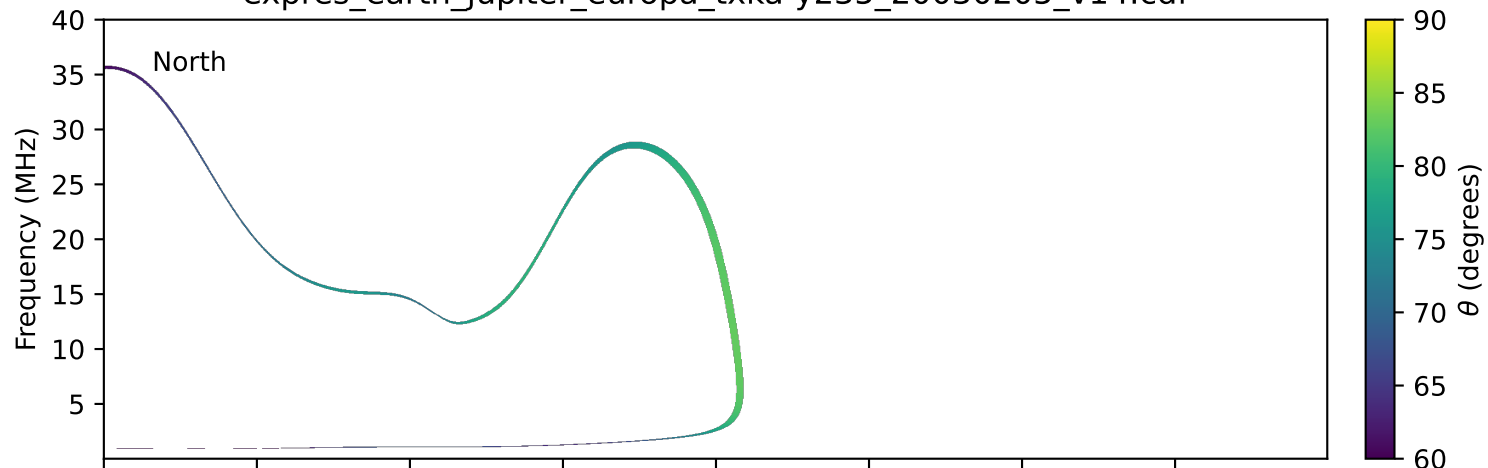
expres_earth_jupiter_europa_txka-y235_20030205_v14.cdf
