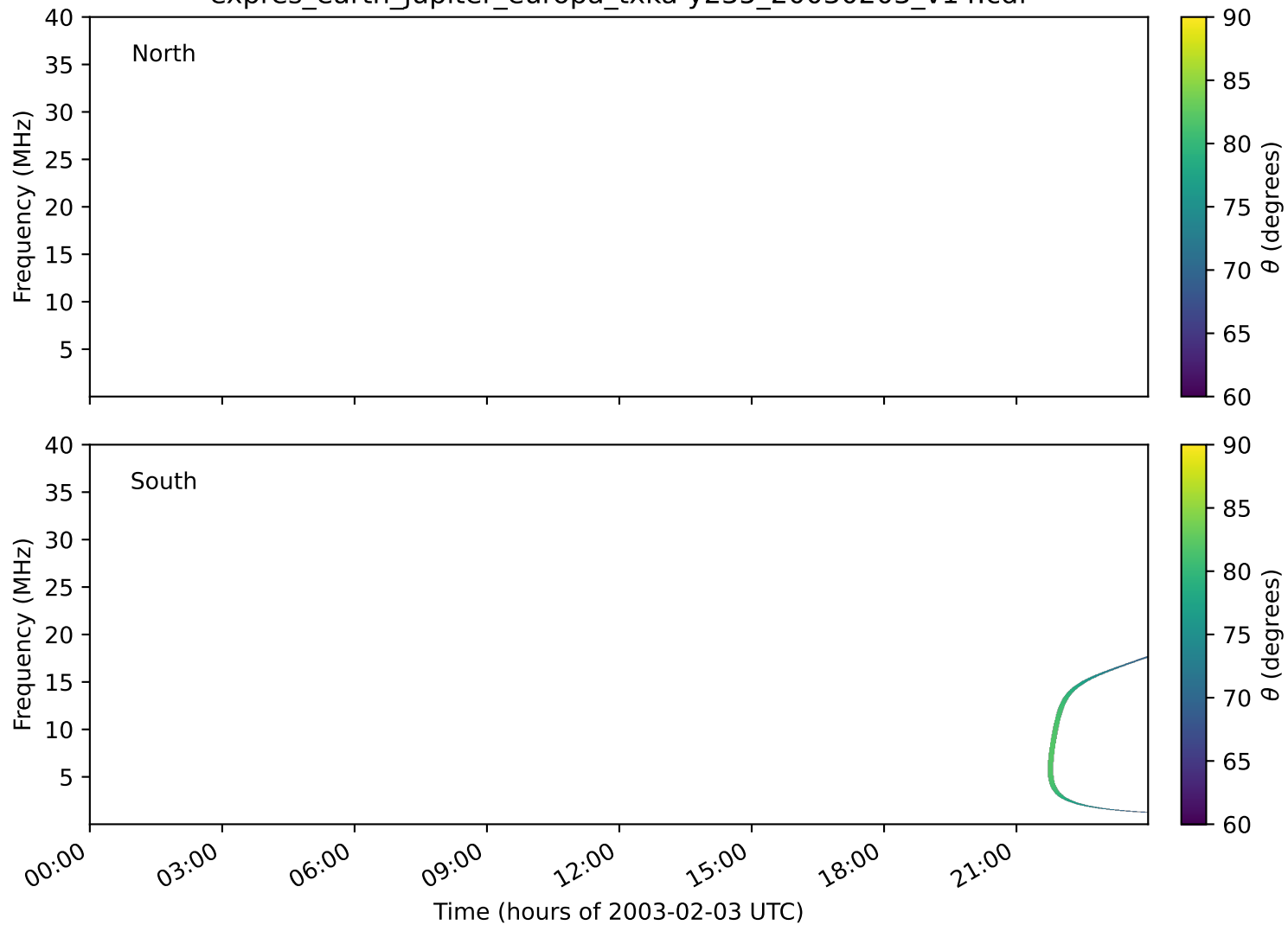
expres_earth_jupiter_europa_txka-y235_20030203_v14.cdf
